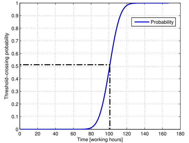
Figure 6: Representation of a risk function: thanks to the properties of the proposed methodology, it is possible to assess the risk of crossing the threshold \mathcal{H}(t) at a generic future time instant.
