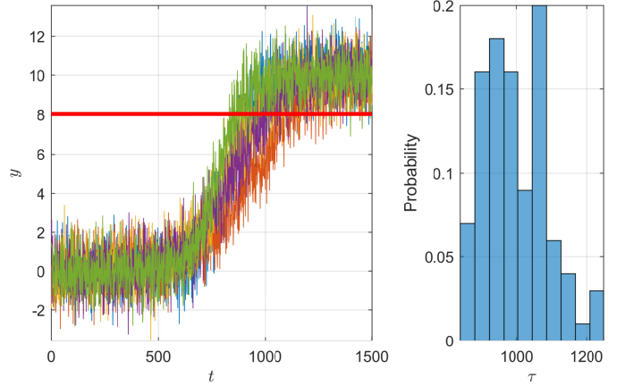
Figure 8: [Sigmoid Data] On the left panel a set of 5 time series from \mathcal{D}^{(1)} is shown. The red line (-) represents the maintenance threshold \mathcal{H} = 8 . On the right panel an histogram of \{\tau_i\}_{i=1}^{100} with \mathcal{H} = 8 .
