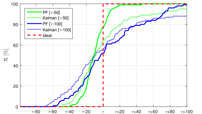
Figure 9: [Sigmoid Data] Averaged Risk Functions associated with different prediction approach and different prediction horizons.
