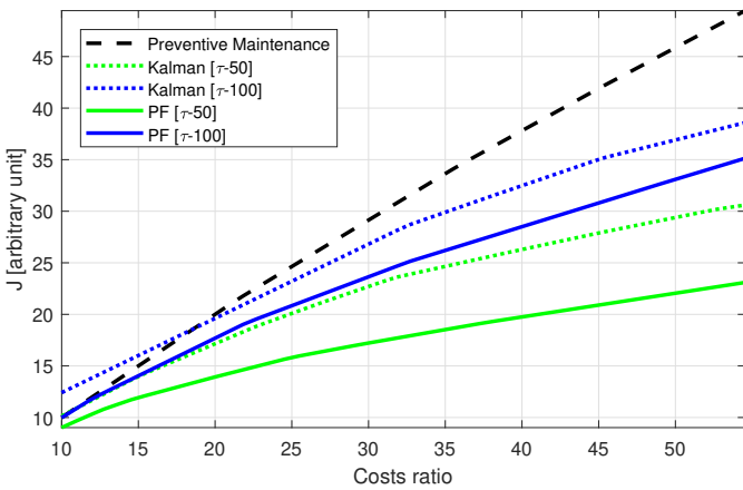
Figure 15: [Industrial Data] Optimal value of J for the various maintenance strategies as a function of the ratio of the costs \frac{c_{UL}}{c_{UB}} (averaged results over 100 Monte Carlo simulations).
