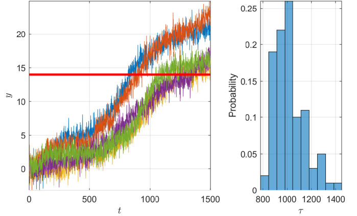
Figure 10: [Sigmoid Data with Discontinuities] On the left panel a set of 5 time series from \mathcal{D}^{(1)} is depicted. The red line (—) represents the maintenance threshold \mathcal{H} = 14 . On the right panel an histogram of \{\tau_i\}_{i=1}^{100} with \mathcal{H} = 14 .
