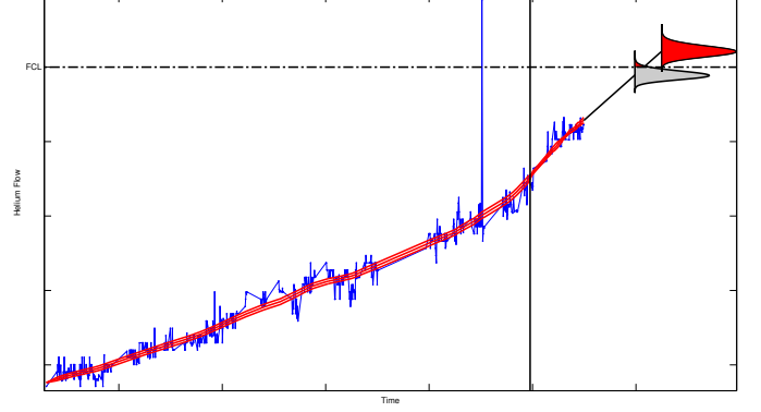
Figure 13: [Industrial Data] Filtering and prediction of the signal presented in Fig. 12.
