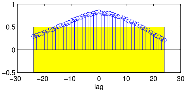
Cross corr. function between input u23 and residuals from output y1
