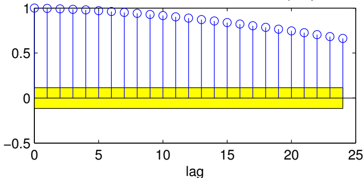
Cross corr. function between input u1 and residuals from output y1
