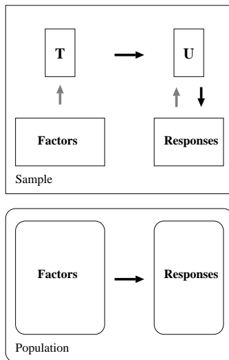
Figure 3: Indirect modeling
