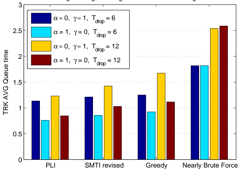
"Tracking" Average Waiting Time for the different algorithms.
