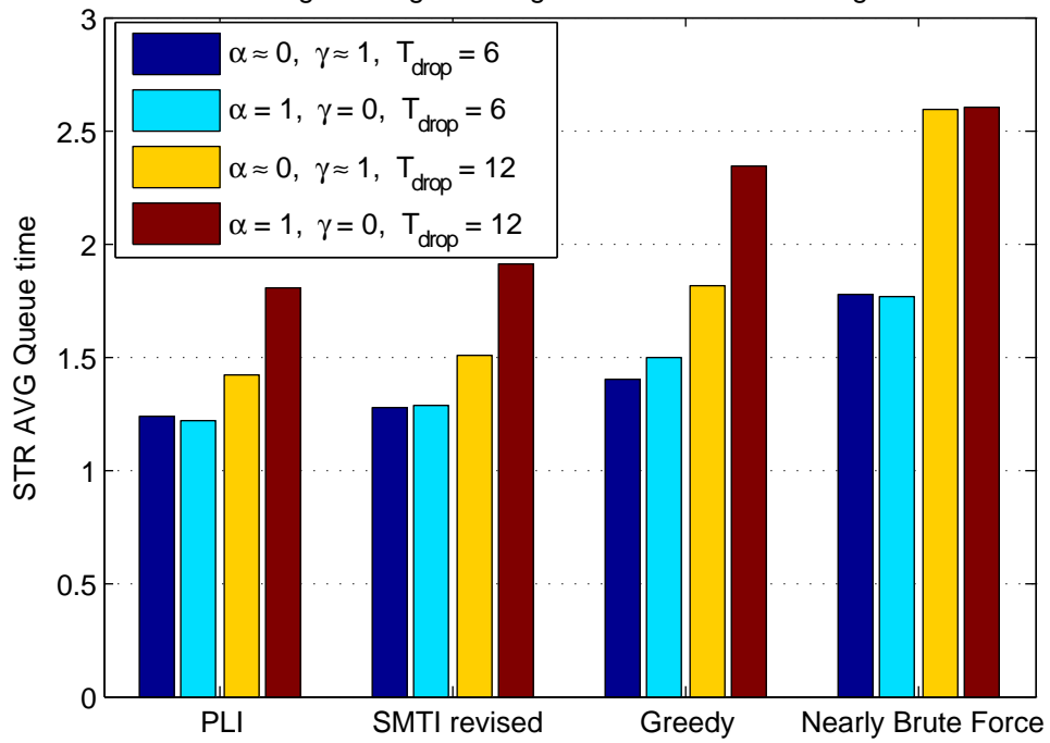
"Streaming" Average Waiting Time for the different algorithms.
