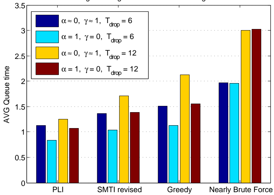
Average Waiting Time for the different algorithms.
