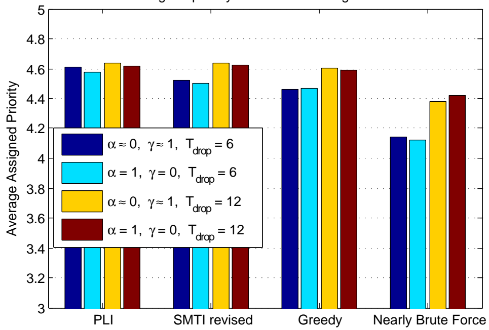
Assigned priority for the different algorithms.
