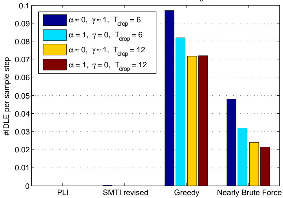
IDLE occurrence for the different algorithms.
