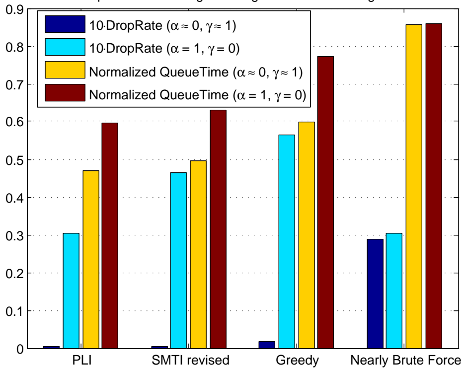
Drop Rate VS Average Waiting Time for Streaming Tasks
