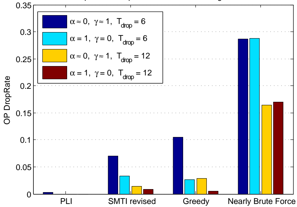
"Operator" Drop Rate for the different algorithms.
