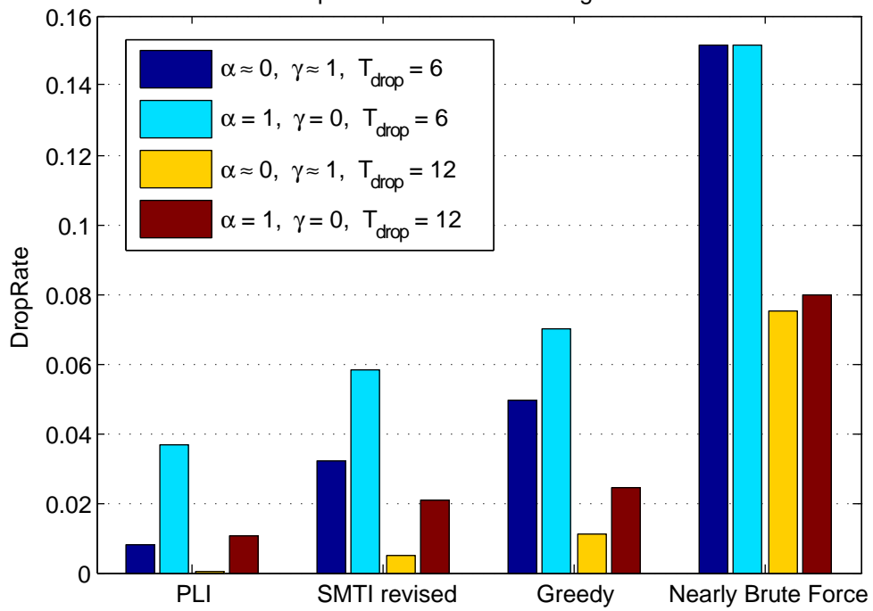
Drop Rate for the different algorithms.
