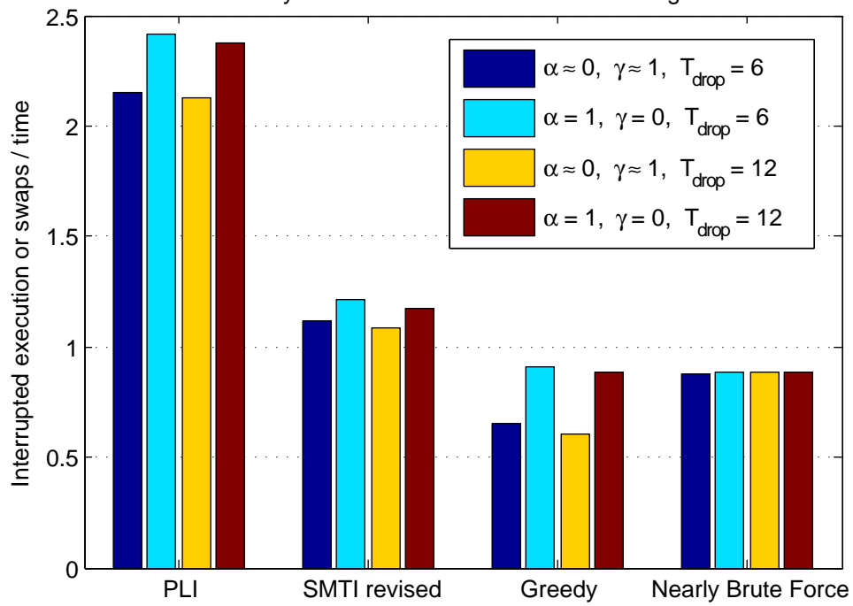
Discontinuity in task execution for the different algorithms.
