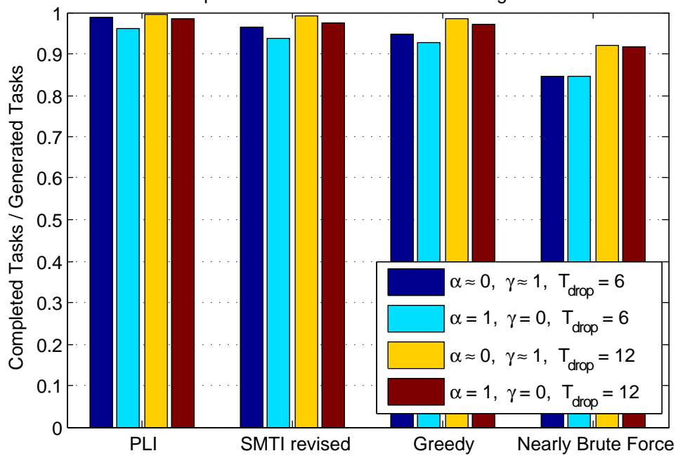
Completed Task Rate for the different algorithms.
